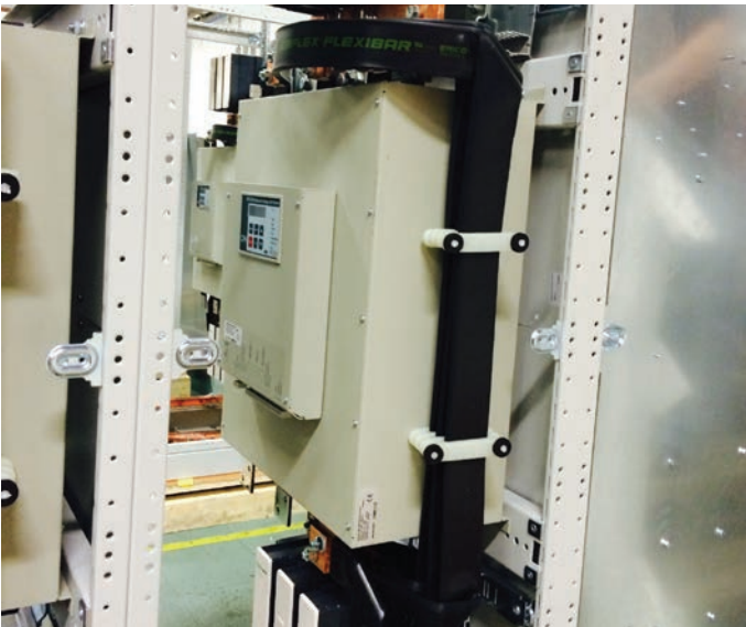
Application pictures: Flexibar fixed/secured with nVent ERIFLEX spacers, clamps and tie.
