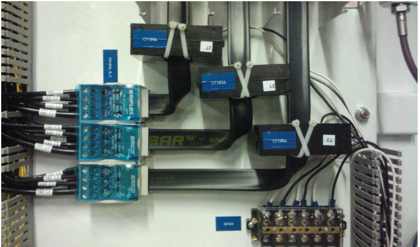
Application pictures: Flexibar directly connected on nVent ERIFLEX Power blocks and Distribution blocks.
